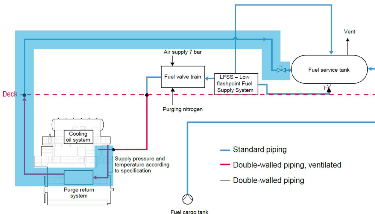
Figure 5-5 Handling and processing of methanol after the main engine, ref. /20/.
