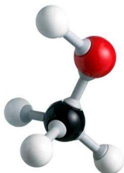
Figure 2-1 Symbolic representation of methanol molecule, \text{CH}_3\text{OH}
