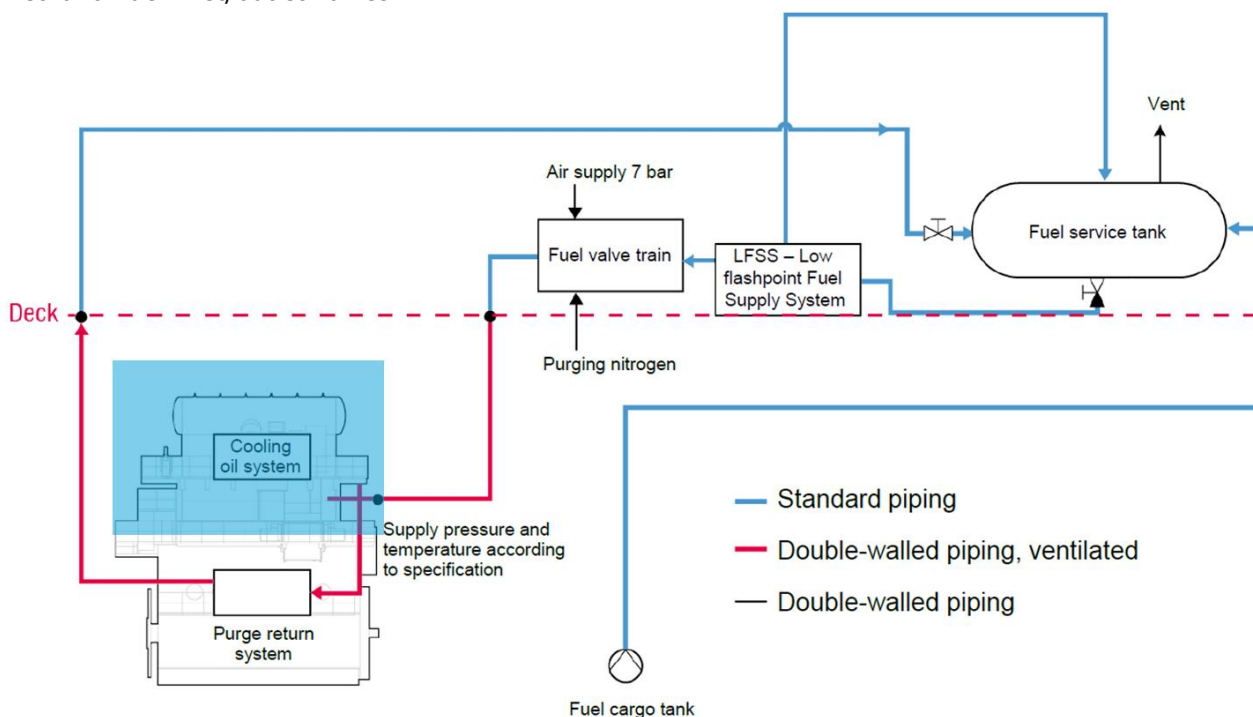
Figure 5-4 Combustion of Methanol in the main engine, ref. /20/
