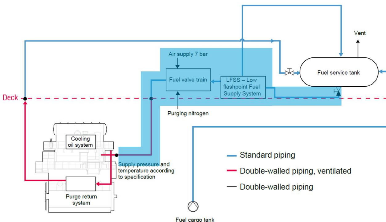
Figure 5-3 Handling and processing of Methanol towards the main engine, ref. /20/
