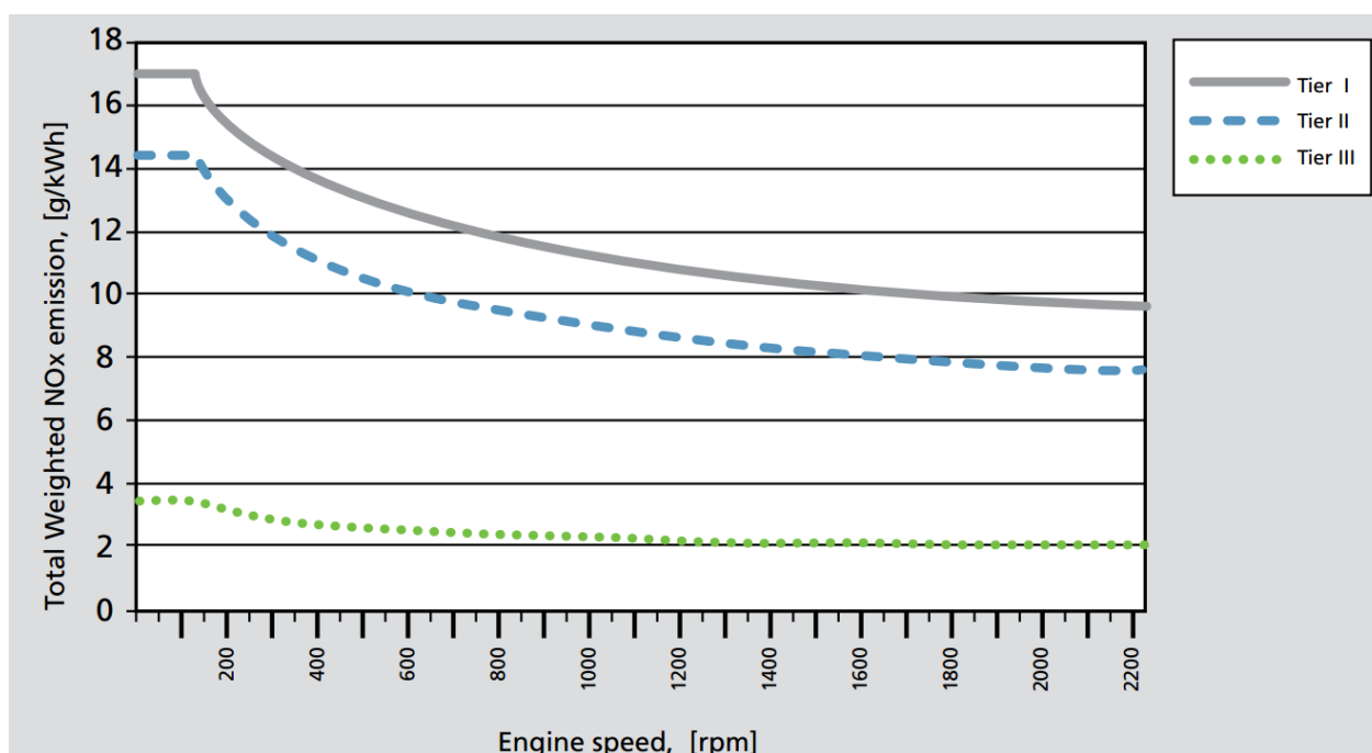
Figure 3-2 Allowable NO x emission from marine engines according to tier
