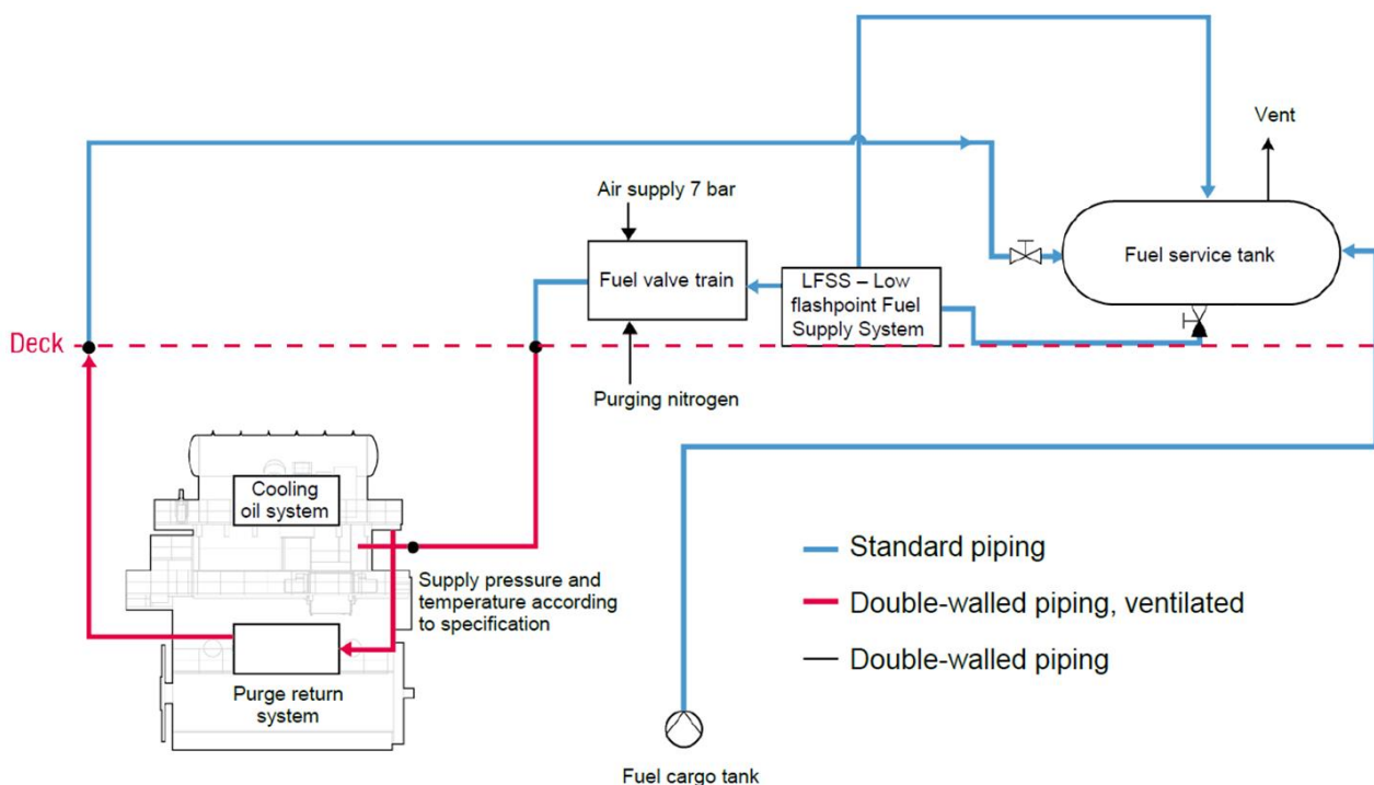
Figure 5-1 Schematic overview of the methanol fuel system, ref. /20/
