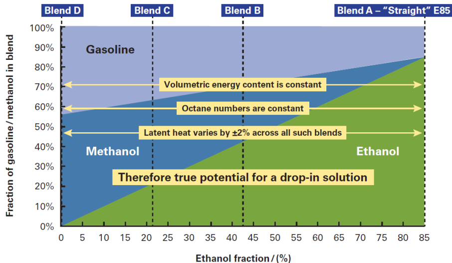
Figure 15: GEM Fuel Blend Testing Results
