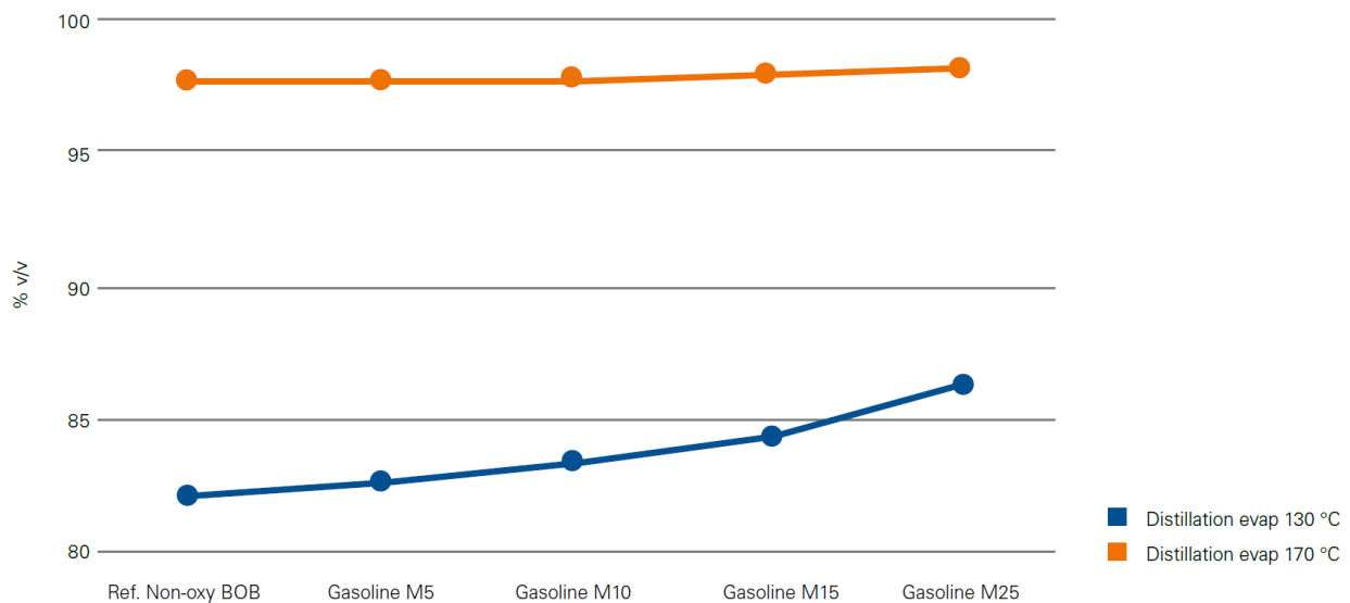
Figure 7: Distillation Evaporation Values for Gasoline and Methanol
