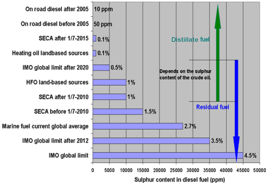
Figure 11. Sulphur Content of Conventional Marine Fuels (Source: Ref. 4)
